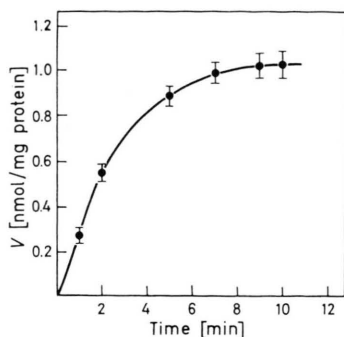
Fig. 1. Time course of synaptosomal uptake of sulphate. Synaptosomes were incubated with 10 mM \text{Na}_2\text{SO}_4 (see text) at 25 °C. Means and standard deviations are given ( n=10 ).
